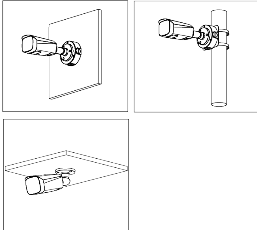
Figure 3-3 Installation methods
