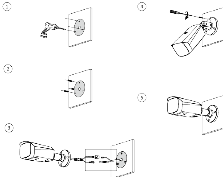
Figure 3-6 Cable going through the mounting surface
